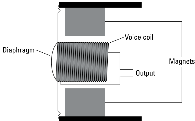
Figure 6-5: Dynamic mics pick up a signal using a magnetic field and a voice coil.
