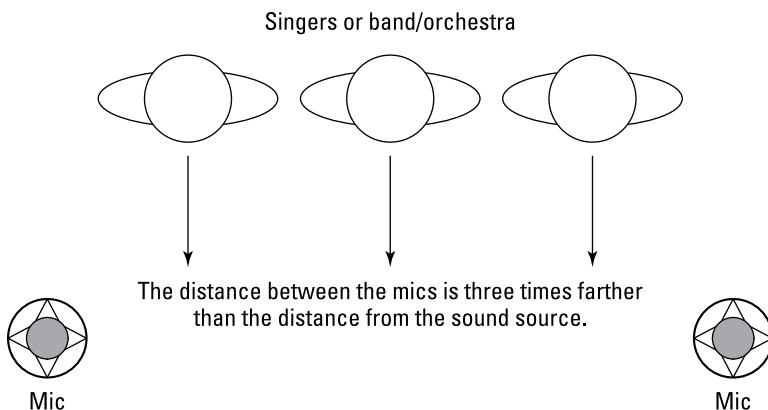
Figure 8-6: To use the spaced-pair approach, place two mics away from the sound source and apart from one another.
