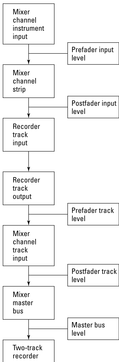
Figure 7-2: Most recording systems allow you to monitor your signal levels at various places in the signal chain.
