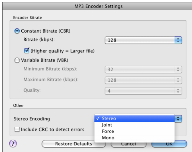
Figure 17-2: MP3 encoders have several modes from which you can choose.
